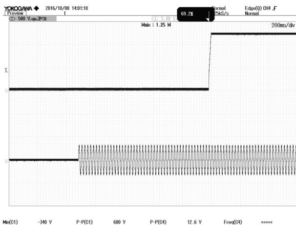
Figure 5: V_{out} start up with Enable on at 220Vac, 25A I_{out} , TOP: V_{out} , 5V/div, 200ms/div BOTTOM: V_{in} , 500V/div, 200ms/div
