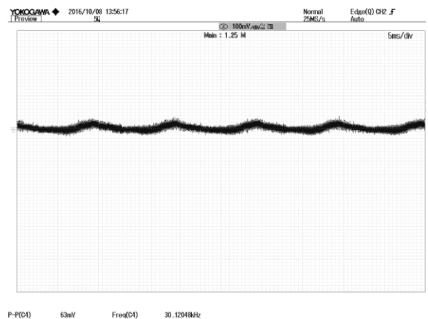
Figure 6: Output ripple & noise at 110/220Vac, 25A I_{out} VOUT: 100mV/div, 5ms/div
