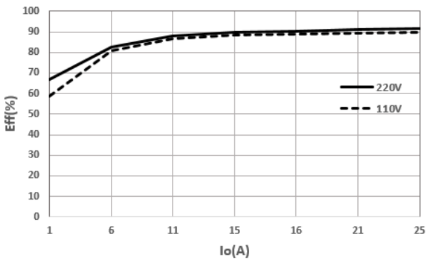
Figure 1: Efficiency vs. Output current @ V_{in}=110,220VAC
