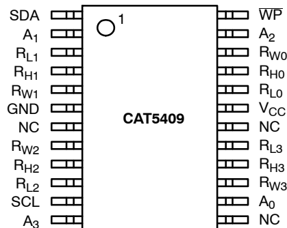
TSSOP-24 (Y) (Top View)
