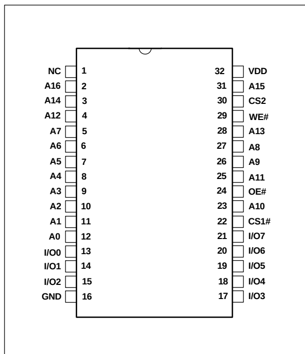
32-Pin SOP
