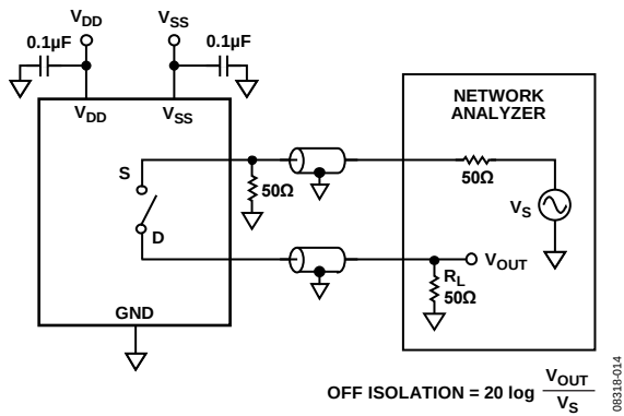
Figure 32. Off Isolation
