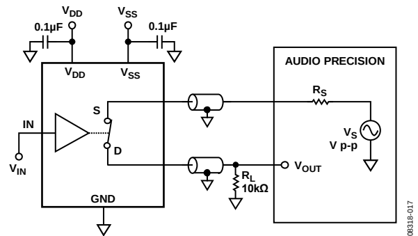
Figure 35. THD + Noise
