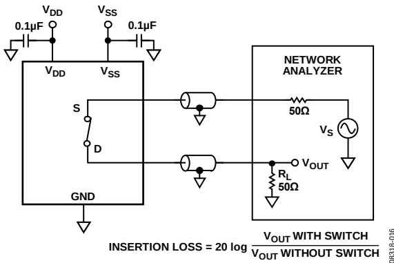
Figure 33. Bandwidth
