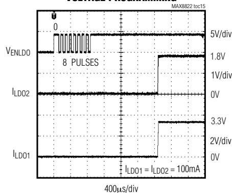
SERIAL-PULSE CONTROL LDO VOLTAGE PROGRAMMING
