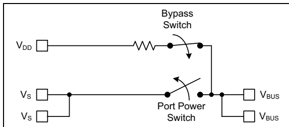
FIGURE 6-1: Bypass Switch.
