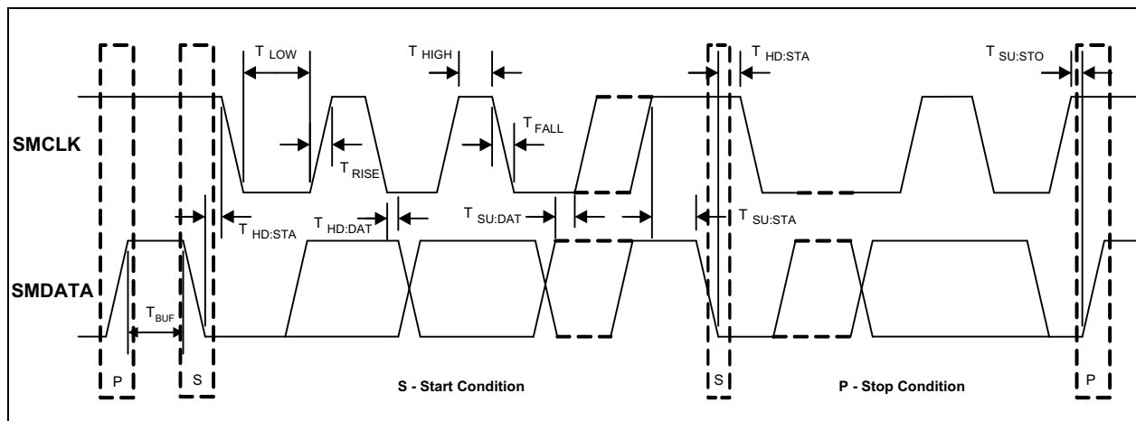
FIGURE 1-1: SMSBus Timing.
