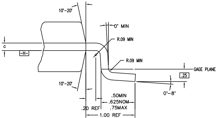
DETAIL B
