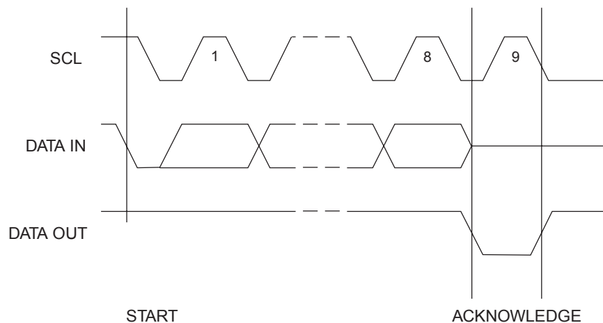
Figure 4-5. Output Acknowledge
