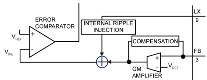
Figure 7. Internal Ripple Injection
