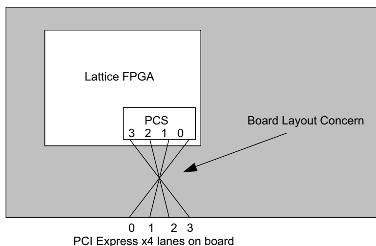
Figure 5-8. Example of Board Layout Concern with x4 Link
