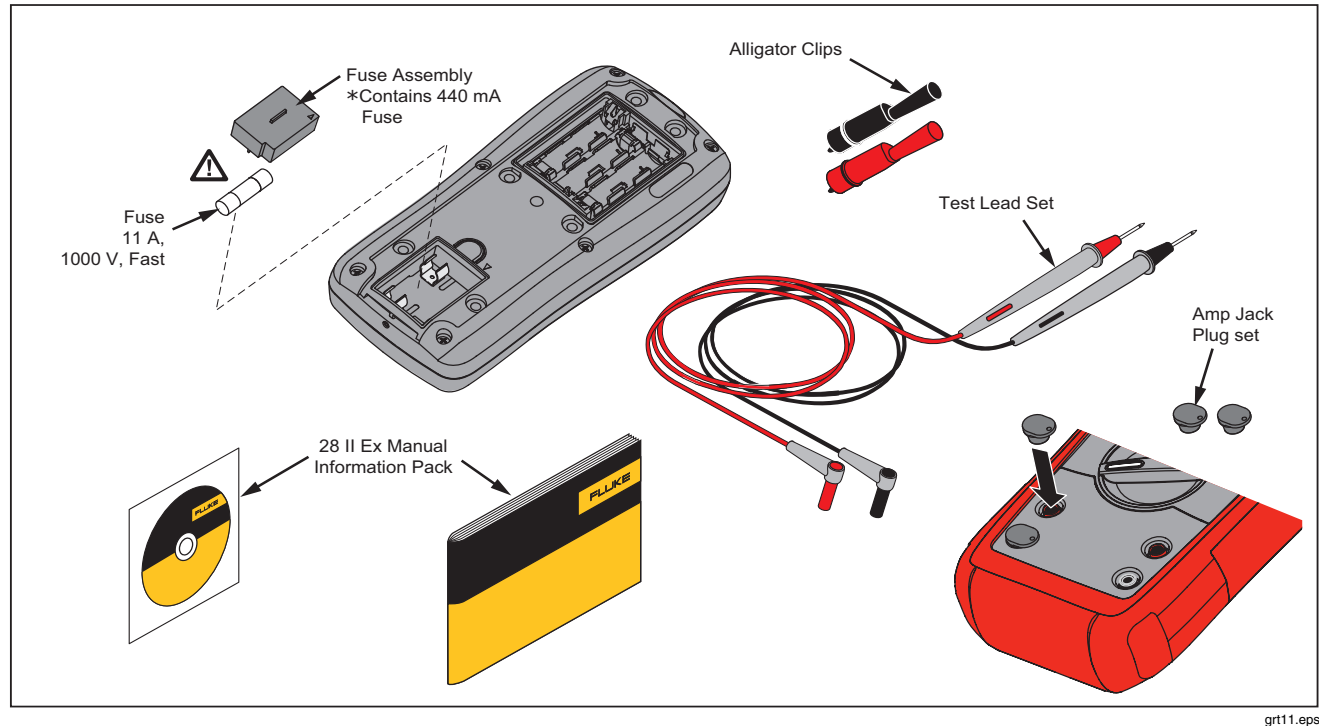
Figure 12. Replacement Parts
