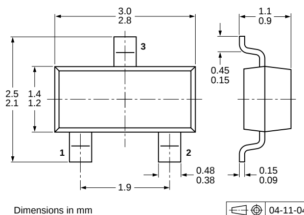
Fig 25. Package outline PDTD1xxxT series (SOT23/TO-236AB)
