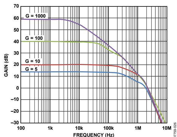
Figure 26. Gain vs. Frequency, V_s = 2.7V
