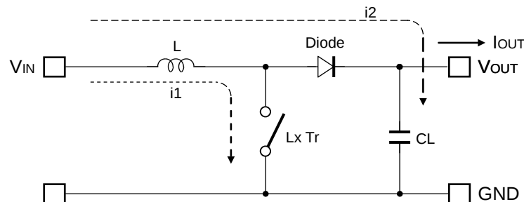
<Basic Circuit>
