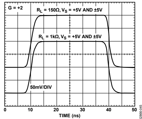
Figure 45. Small Signal Transient Response for R_L = 150\Omega , R_L = 1k\Omega and V_S = +5V , V_S = \pm 5V
