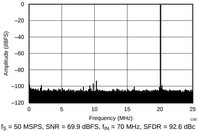
Figure 102. FFT for 70-MHz Input Signal (Dither On)
