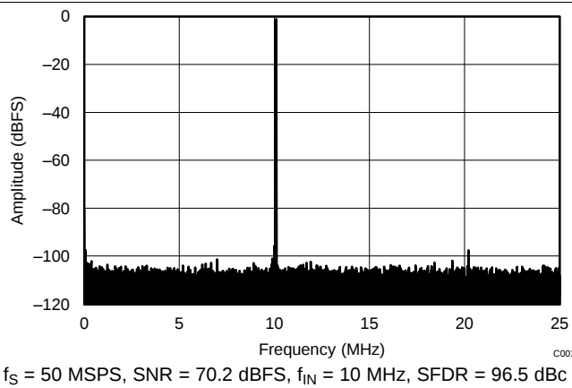
Figure 100. FFT for 10-MHz Input Signal (Dither On)
