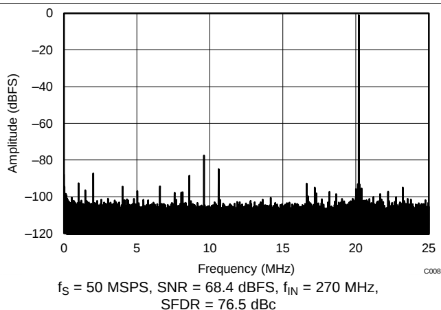
Figure 107. FFT for 270-MHz Input Signal (Dither Off)
