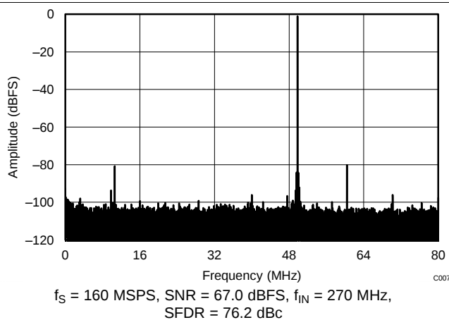
Figure 7. FFT for 270-MHz Input Signal (Dither On)
