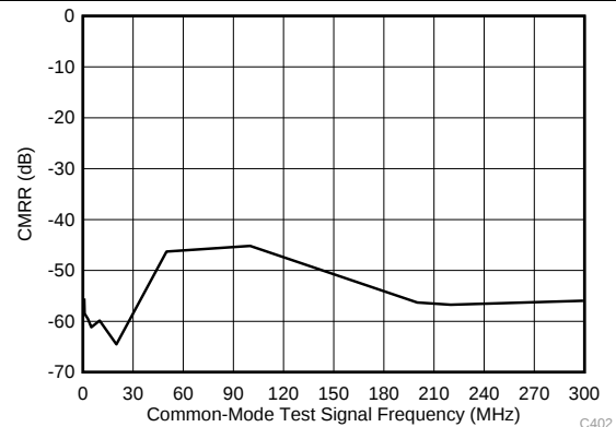
Figure 134. Common-Mode Rejection Ratio vs Test Signal Frequency
