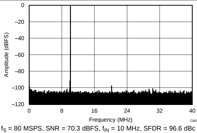
Figure 67. FFT for 10-MHz Input Signal (Dither On)
