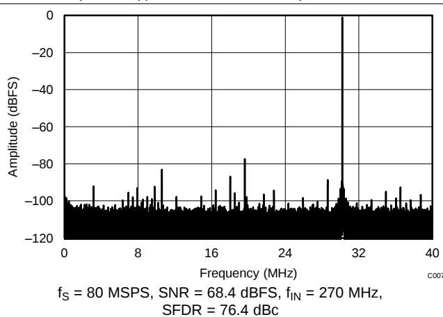
Figure 73. FFT for 270-MHz Input Signal (Dither On)
