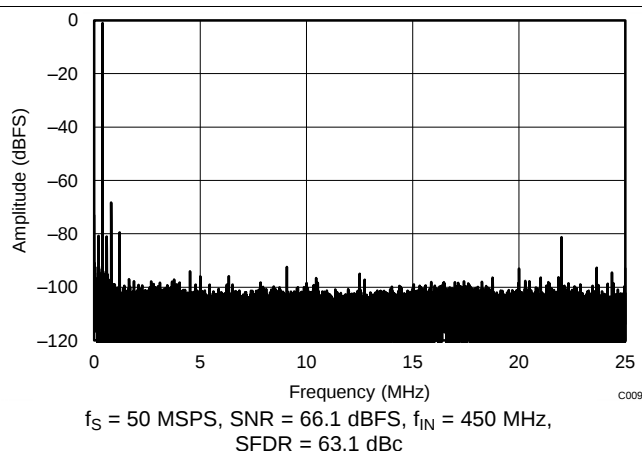
Figure 108. FFT for 450-MHz Input Signal (Dither On)
