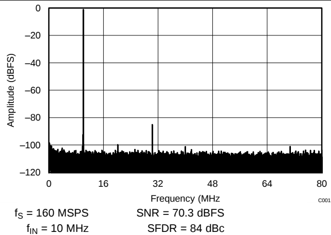
Figure 203. Performance FFT at 10 MHz (Low Input Frequency)
