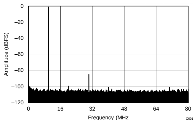
FFT with Dither On ( f_s = 160 MSPS, f_{IN} = 10 MHz, SNR = 70.3 dBFS, SFDR = 84 dBc)
