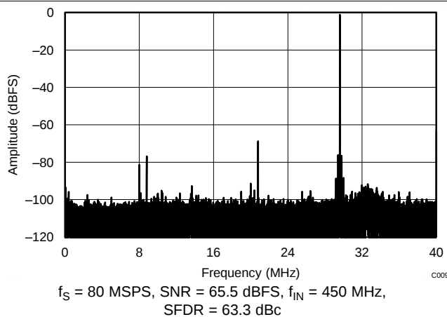
Figure 75. FFT for 450-MHz Input Signal (Dither On)
