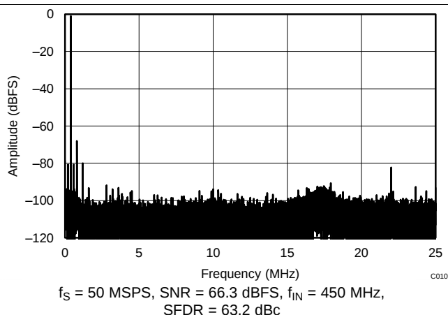
Figure 109. FFT for 450-MHz Input Signal (Dither Off)
