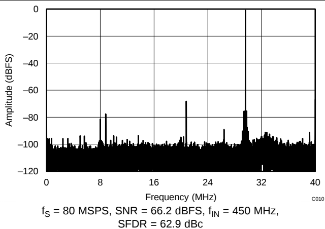
Figure 76. FFT for 450-MHz Input Signal (Dither Off)
