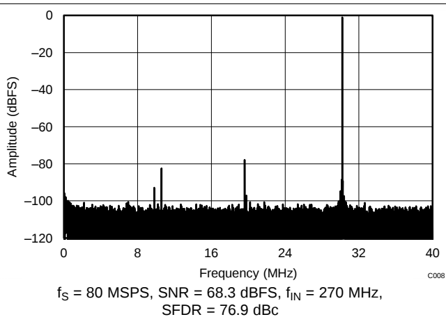
Figure 74. FFT for 270-MHz Input Signal (Dither Off)
