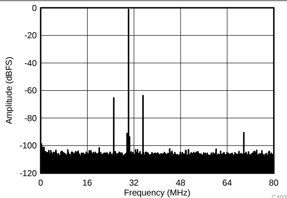
Figure 133. Common-Mode Rejection Ratio FFT
