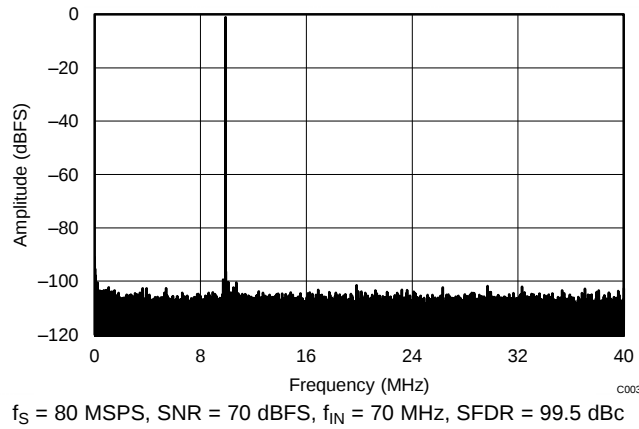
Figure 69. FFT for 70-MHz Input Signal (Dither On)
