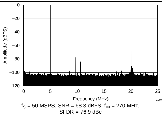
Figure 106. FFT for 270-MHz Input Signal (Dither On)
