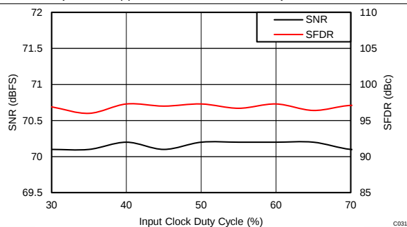
Figure 97. Performance vs Clock Duty Cycle (40 MHz)
