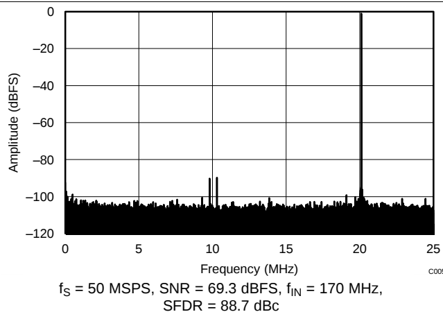
Figure 104. FFT for 170-MHz Input Signal (Dither On)
