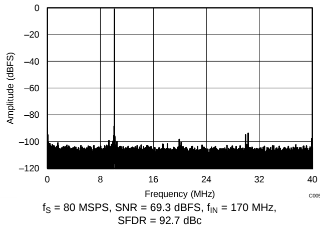
Figure 71. FFT for 170-MHz Input Signal (Dither On)
