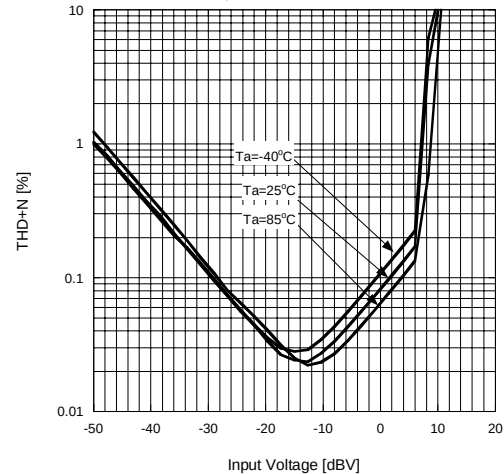
THD+N vs. Input Voltage (eala)
