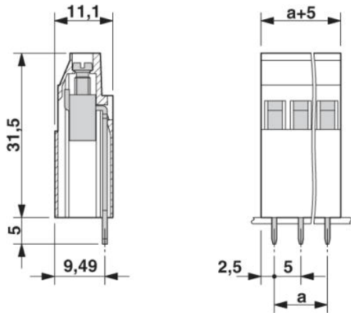
Dimensioned drawing
