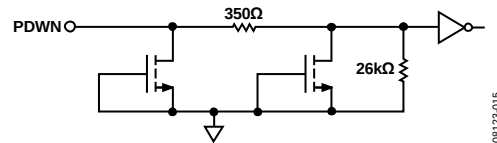
Figure 63. Equivalent PDWN Input Circuit
