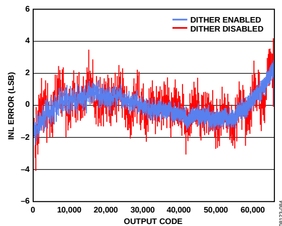
Figure 30. AD9268-105 INL with f_{IN} = 9.7 MHz
