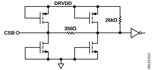
Figure 61. Equivalent CSB Input Circuit
