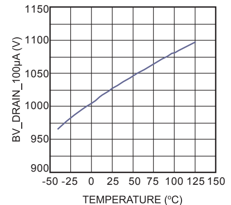
BV_Drain_100µA vs. Temperature
