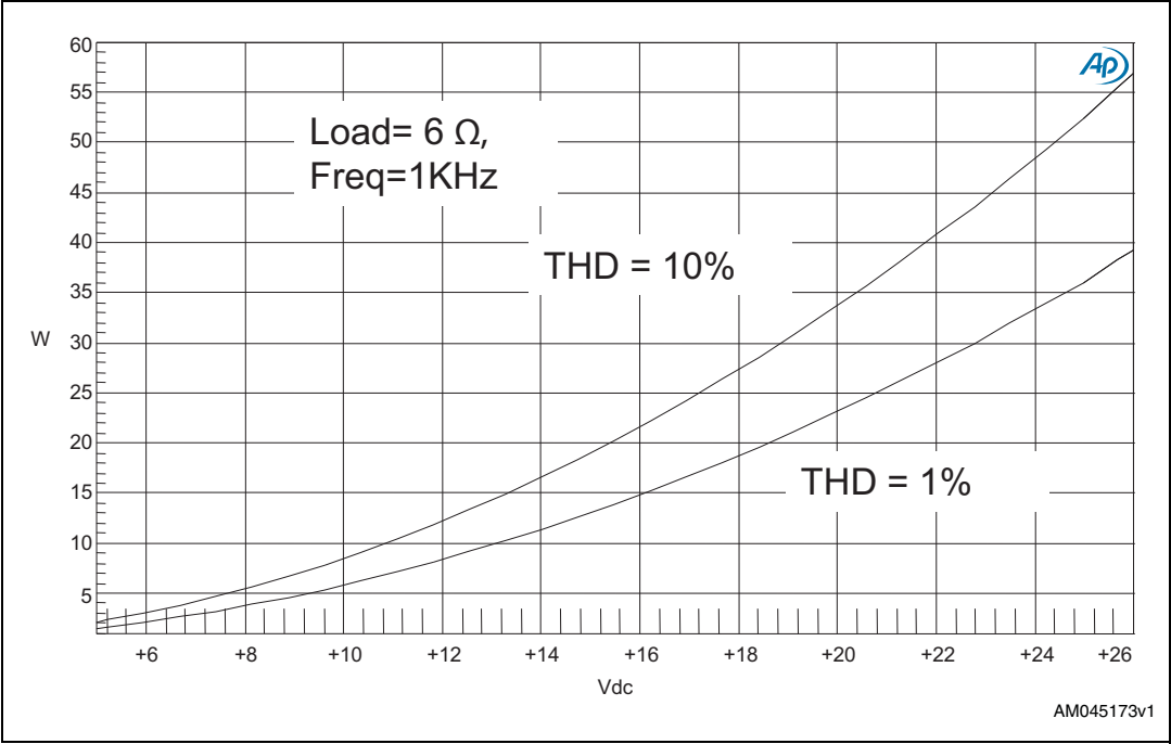
Figure 10. Output power vs. V_{CC} (load = 6 \Omega )
