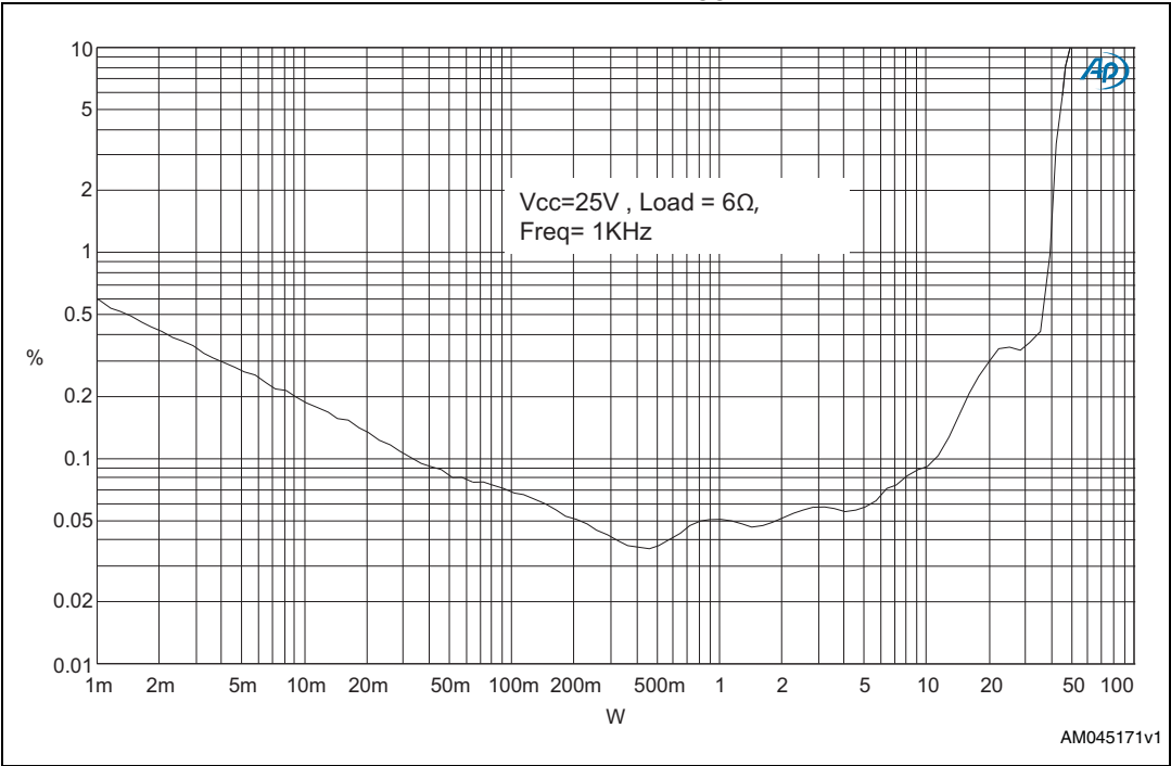
Figure 8. THD+N vs. output power ( V_{CC} = 25\text{ V} , load = 6\ \Omega )
