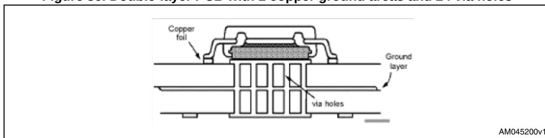
Figure 36. Double-layer PCB with 2 copper ground areas and 24 via holes
