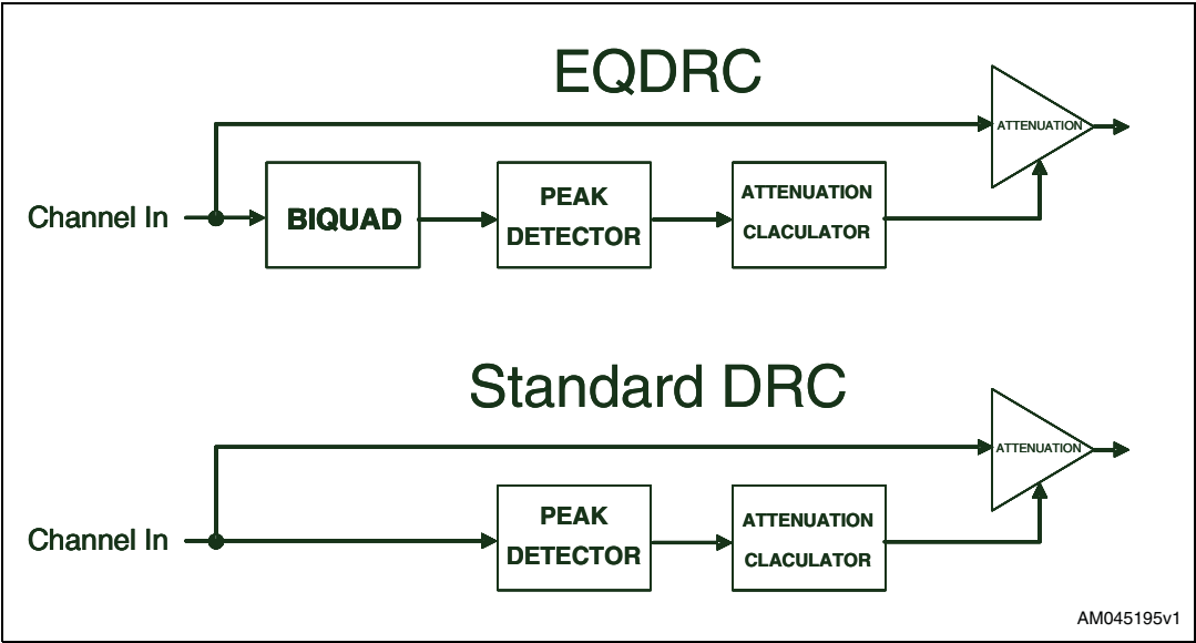
Figure 33. EQDRC scheme
