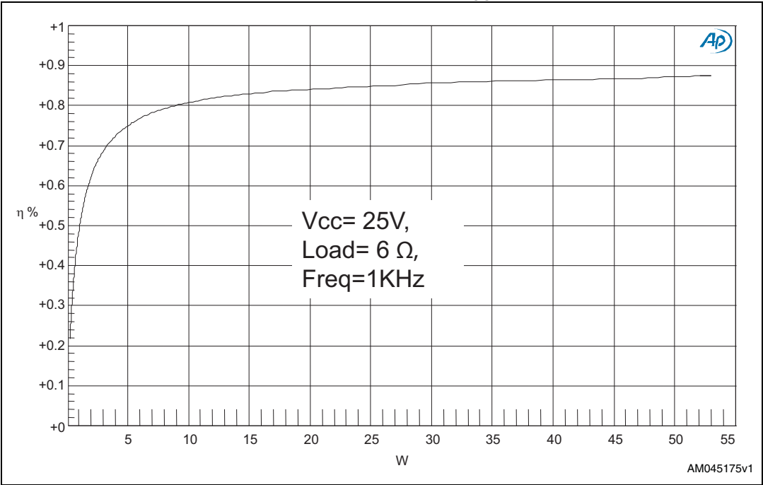
Figure 12. Efficiency vs. output power ( V_{CC} = 25\text{ V} , load = 6\ \Omega )
