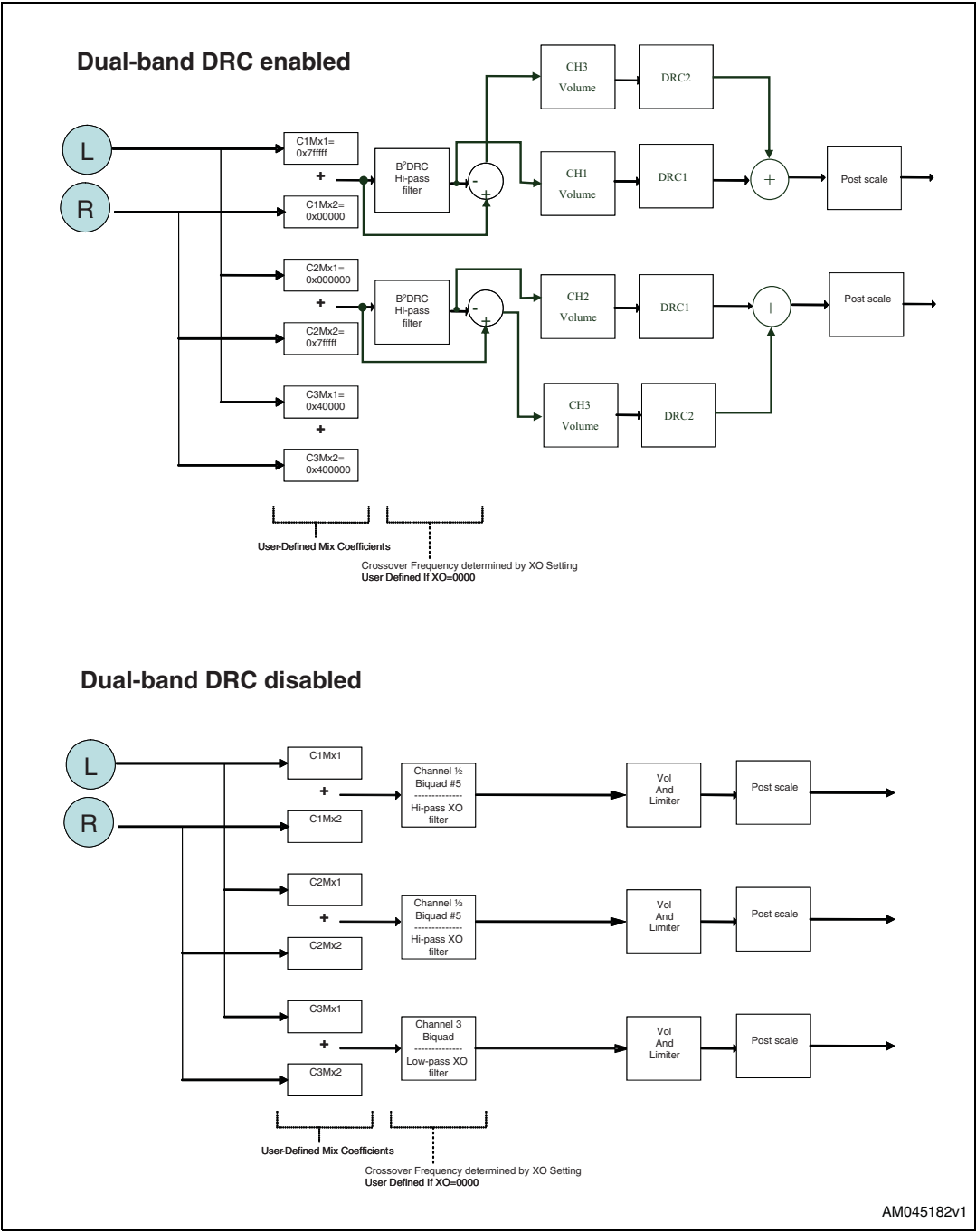
Figure 20. Processing - part 2
