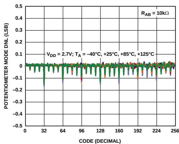
Figure 9. DNL vs. Code vs. Temperature
