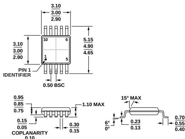
COMPLIANT TO JEDEC STANDARDS MO-187-BA Figure 50. 10-Lead Mini Small Outline Package [MSOP] (RM-10)
