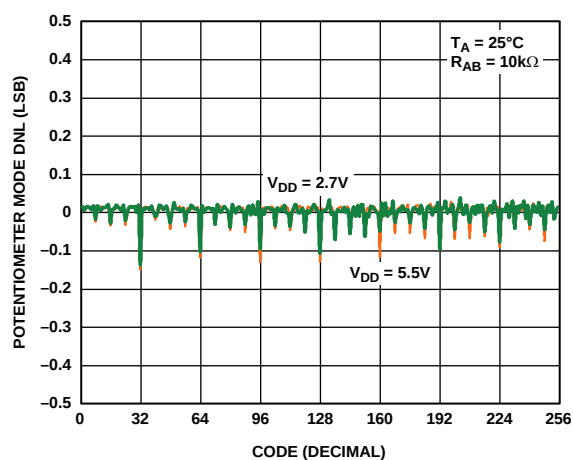
Figure 11. DNL vs. Code vs. Supply Voltages
