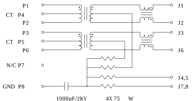
PCB
