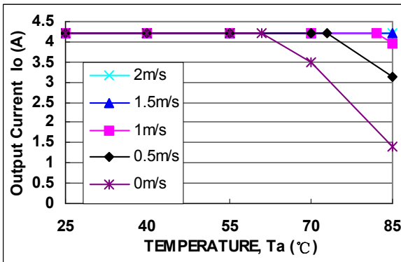
Fig.89 AVO50-48S12 output power derating Airflow direction from -VIN to +VIN; VIN = 48V
