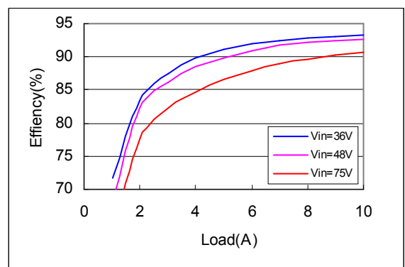
Fig.6 Typical efficiency of AVO50-48S05
