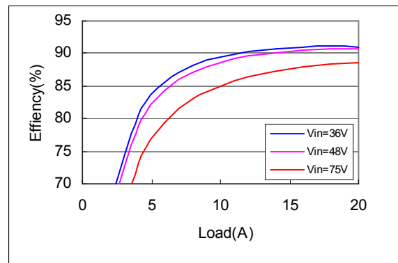
Fig.4 Typical efficiency of AVO50-48S2V5
