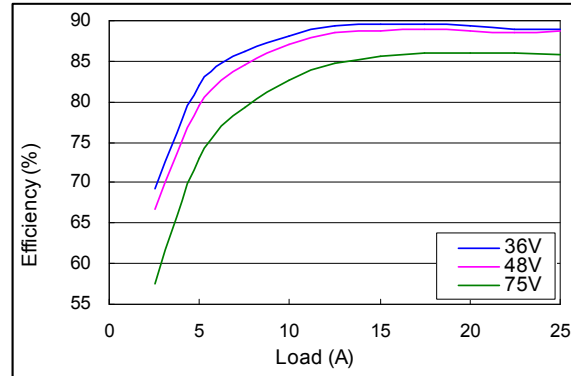
Fig.2 Typical efficiency of AVO50-48S1V5
