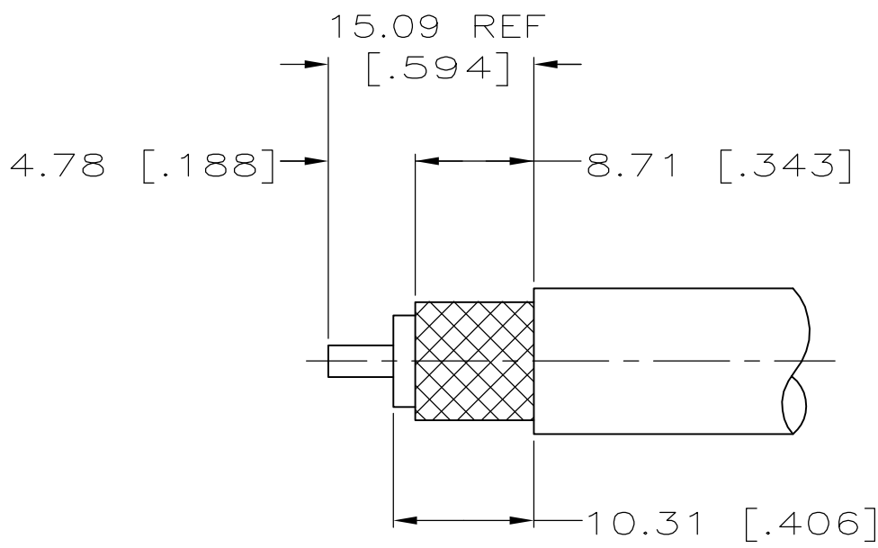
RECOMMENDED STRIP LENGTH SCALE 2:1
