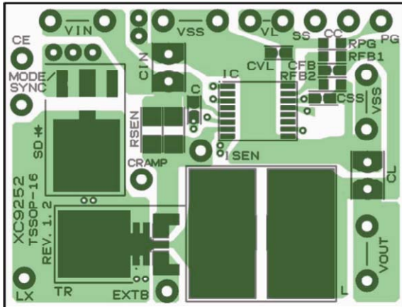
TSSOP-16 (Front)
