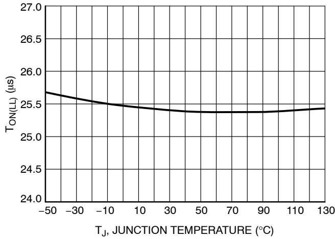
Figure 39. Maximum On Time @ V_{SENSE} = 1.4 V vs. Temperature
