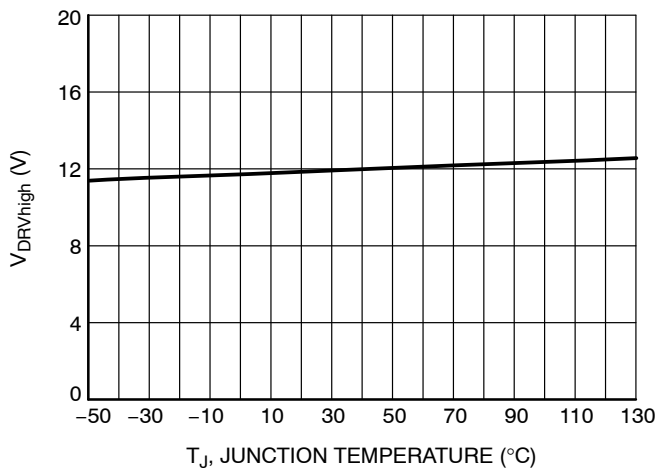
Figure 19. DRV Pin Level @ V_{CC} = 35 V ( R_L = 33 k \Omega , C_L = 1 nF) vs. Temperature
