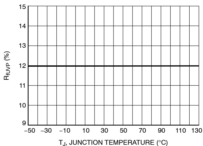
Figure 48. Ratio (UVP Threshold, V_{FB} Rising) over V_{REF} vs. Temperature
