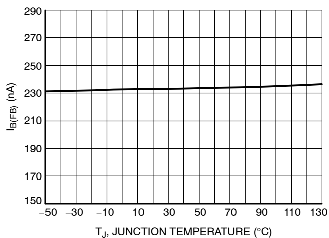
Figure 46. Feedback Pin Bias Current @ V_{FB} = V_{OVP} vs. Temperature
