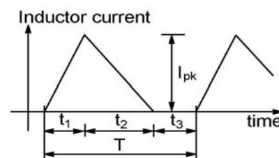
Figure 64. PFC Boost Converter (left) and Inductor Current in DCM (right)
