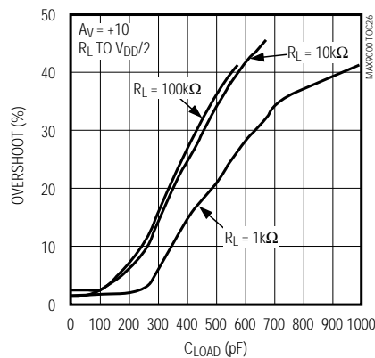
MAX9003/MAX9004/MAX9005 OP-AMP PERCENT OVERTHOOT vs. LOAD CAPACITANCE
