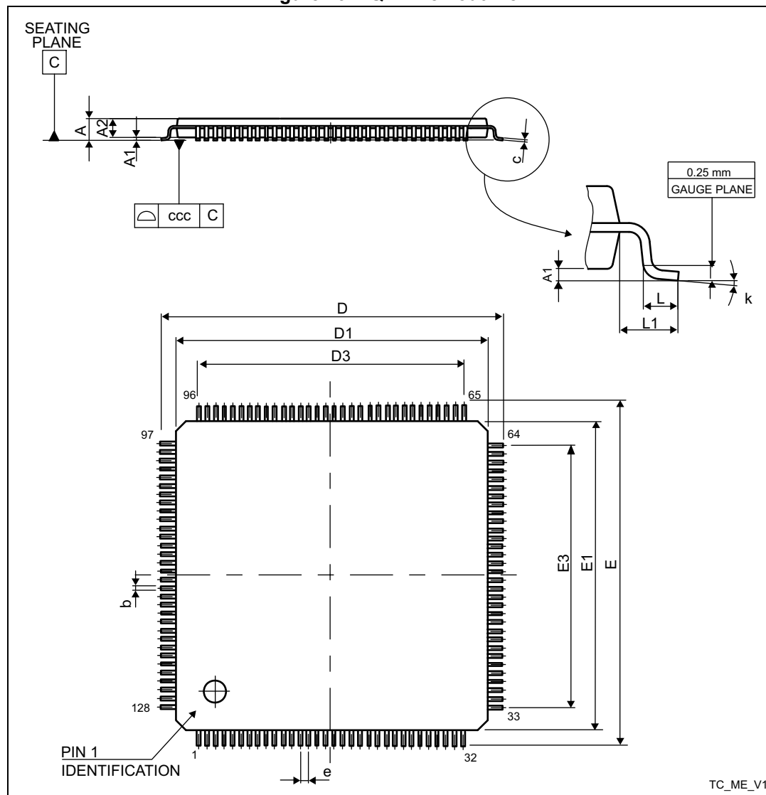
Figure 73. LQFP128 - outline
