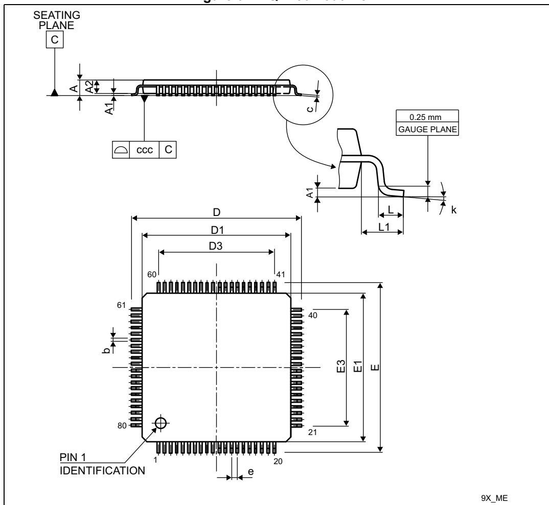
Figure 64. LQFP80 - outline
