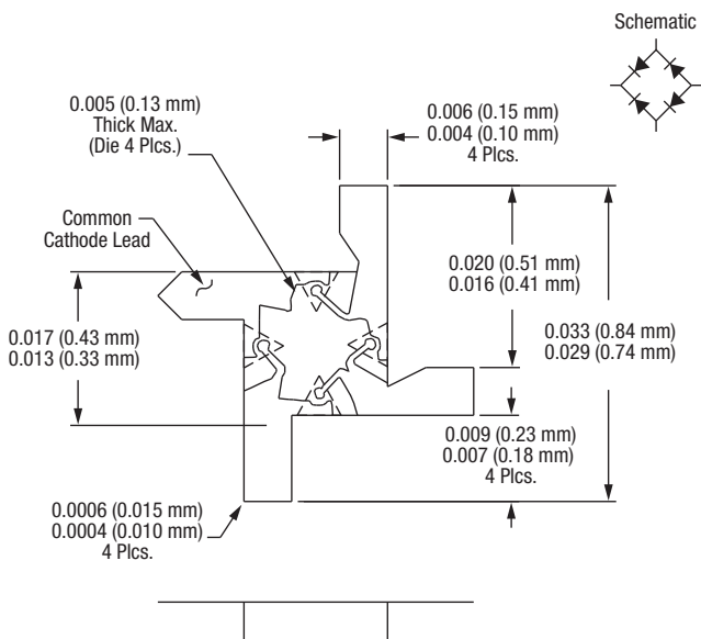
Figure 6. 488-004 Package Dimensions
