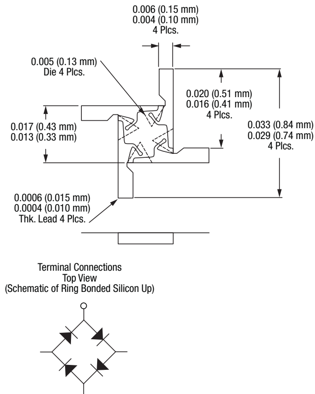
Figure 5. 488-002 Package Dimensions
