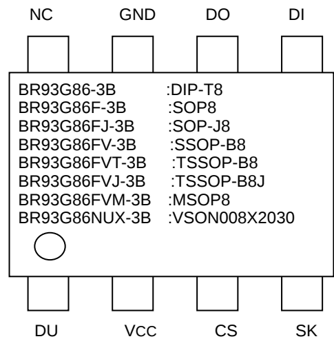
Figure 3. Pin Configuration
