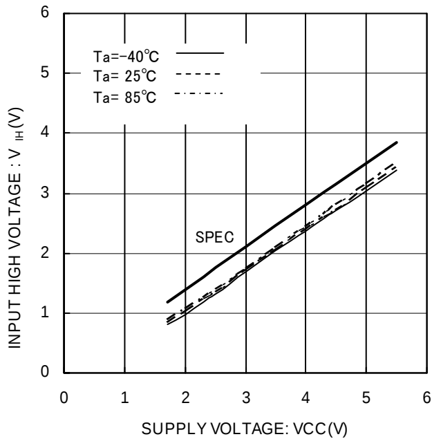
Figure 4. Input high voltage V_{IH}(\text{CS,SK,DI})
