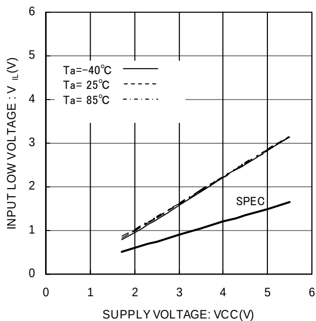
Figure 5. Input low voltage V_{IL}(\text{CS,SK,DI})
