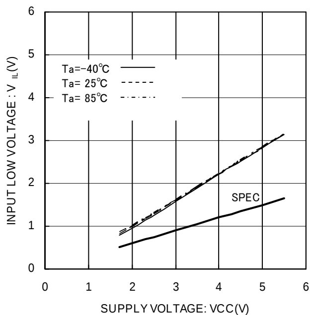
Figure 5. Input low voltage V_{IL} (CS,SK,DI)
