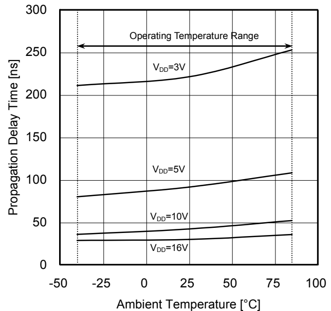
Figure 10. "H" to "L" Propagation Delay Time t_{PLH}
