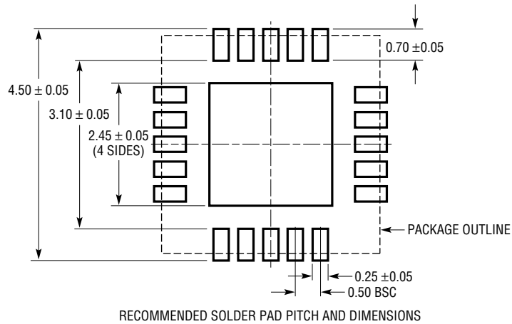
UF Package 20-Lead Plastic QFN (4mm × 4mm) (Reference LTC DWG # 05-08-1710)
