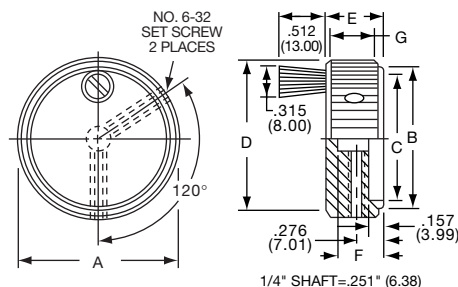
1/4" SHAFT=.251" (6.38)
