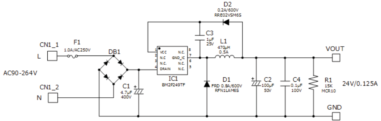
Figure 23. BM2P249TF-EVK-001 Schematics
