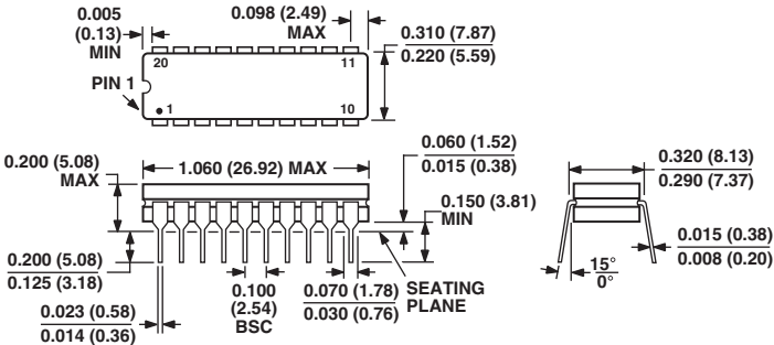
20-Lead Ceramic Dual In-Line Package [CERDIP] (Q-20)
