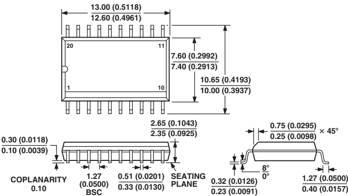
20-Lead Standard Small Outline Package [SOIC] Wide Body (R-20)
