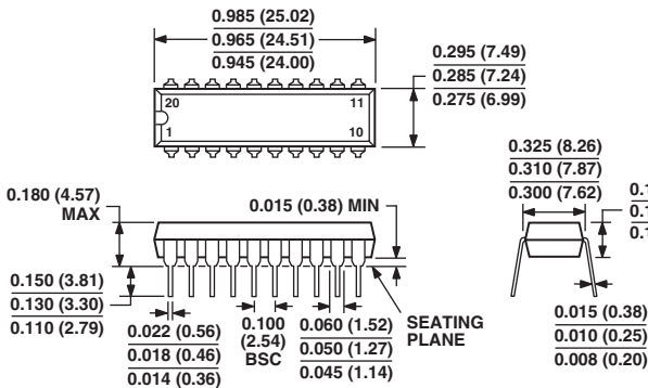
20-Lead Plastic Dual In-Line Package [PDIP] (N-20)
