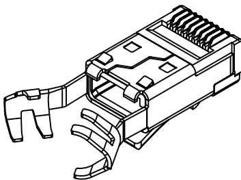
PRE-INSERTED PLUG BODY WITH SHIELD 39200-316
