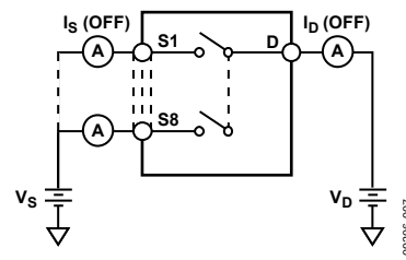
Figure 29. Off Leakage
