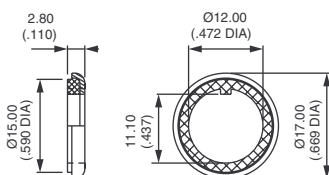
SEALING WASHER
