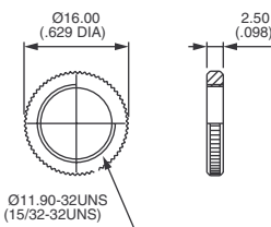
KNURLED NUT
