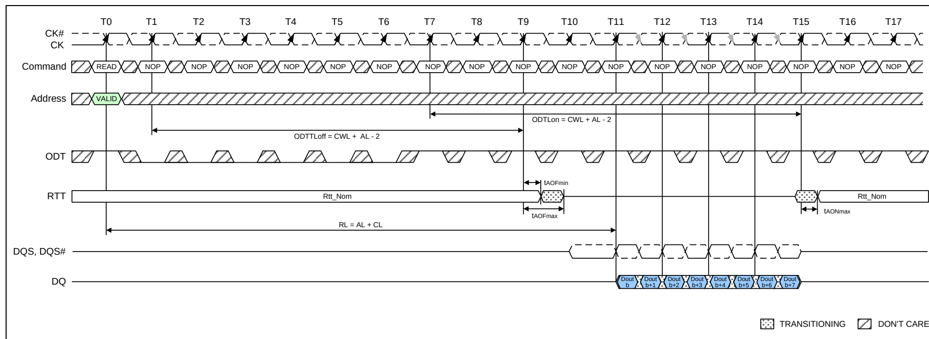
Figure 76 – ODT must be disabled externally during Reads by driving ODT low. (CL = 6; AL = CL - 1 = 5; RL = AL + CL = 11; CWL = 5; ODTLo = CWL + AL - 2 = 8 ; ODTLoff = CWL + AL - 2 = 8 )
