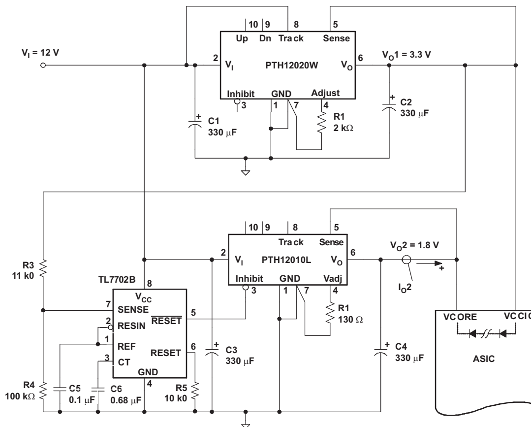
Figure 17. Application Circuit Demonstrating Prebias Startup
